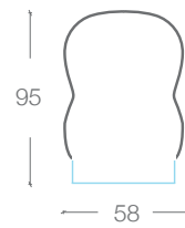
Wave 68 U opal diffuser
